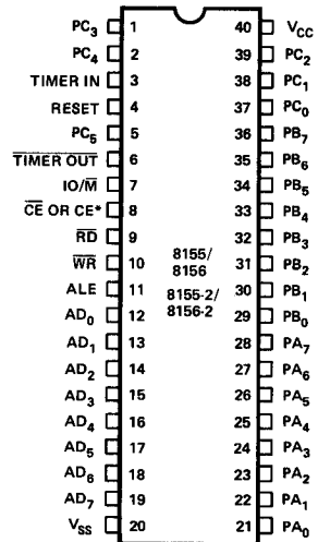
Figure 2. Pin Configuration
