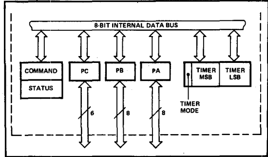
Figure 3. 8155/8156 Internal Registers
