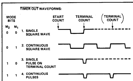
Figure 11. Timer Modes
