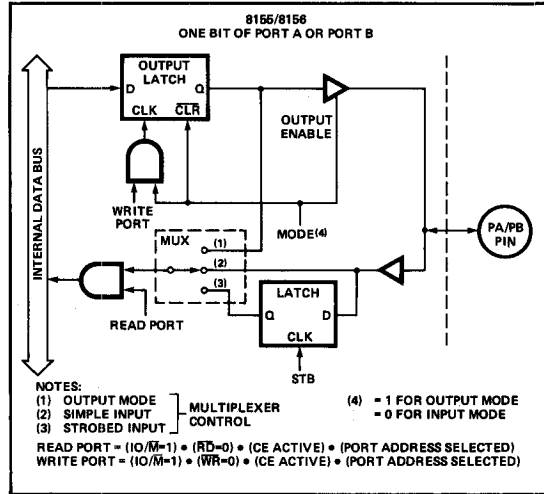
Figure 8. 8155/8156 Port Functions
